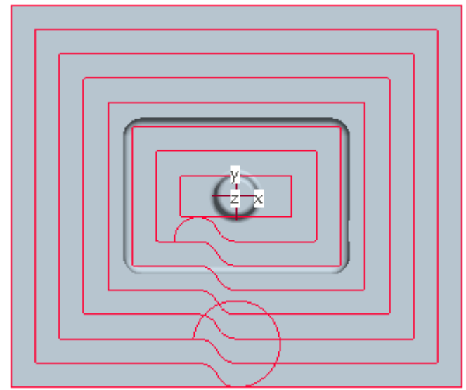
High Speed Facing- Single Entry/Exit, "S" Connection between Passes, Corner Rounding
